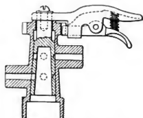
Fig. 3339. Engineer's Valve for Operating Pneumatic Blow-off Cock.
